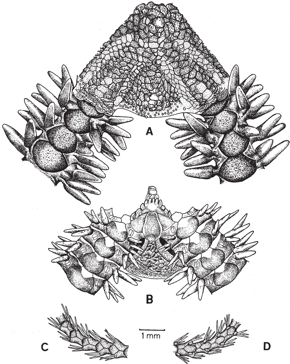
Fig. 1. Ophiocoma similanensis new species. A. Disc, aboral view. B. Disc, oral view. C. Arm tip, aboral view. D. Arm tip, oral view.
